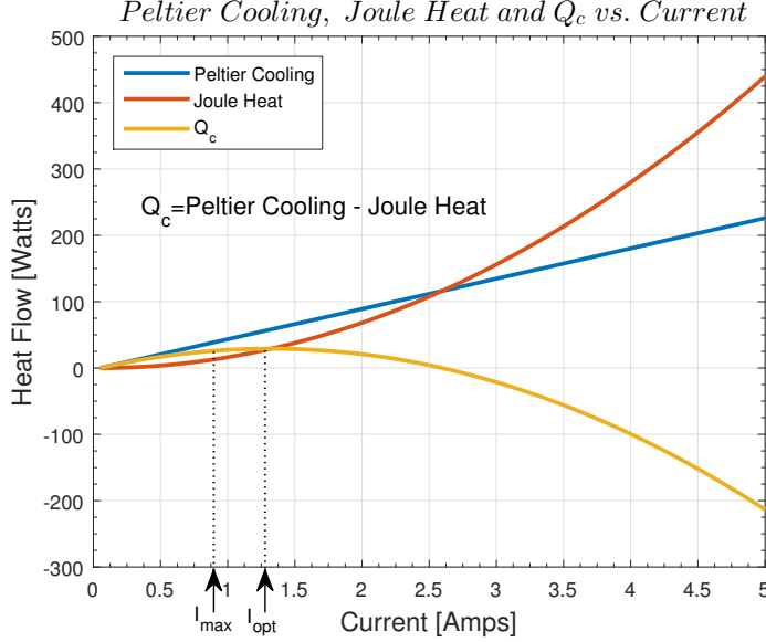
Figure 2.3. Peltier Cooling, Joule Heat and Q_c vs. Current
