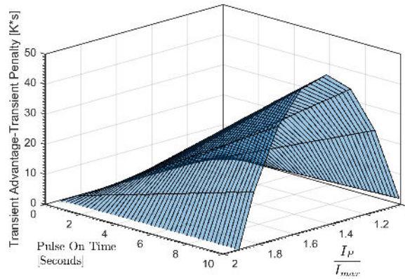
Figure 4.11. Net Transient Advantage - Advantage Portion, I_{max} Surface
