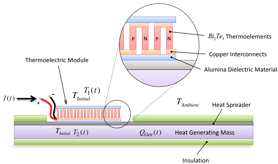
Figure 3.2. System Model
