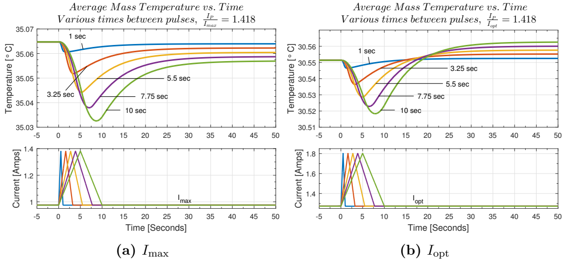
Figure 5.5. Effect of Pulse On-Time to Mass Temperature
