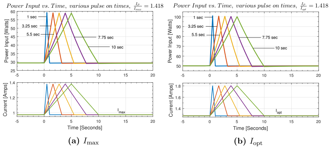
Figure 5.7. Effect of Pulse On-Time on P_{\text{in}}
