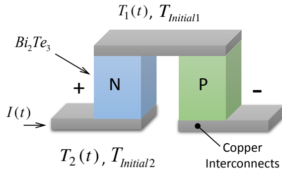
Figure 3.1. Thermocouple
