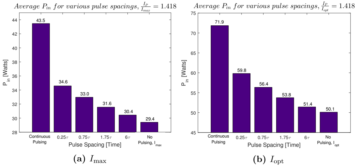
Figure 5.37. Average Effect of Pulse Spacing on P_{in}
