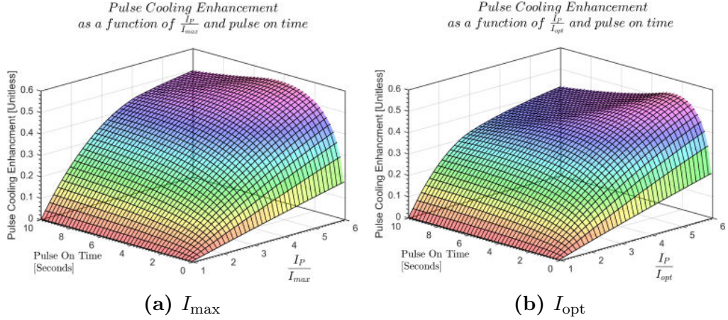
Figure 4.4. Pulse Cooling Enhancement
